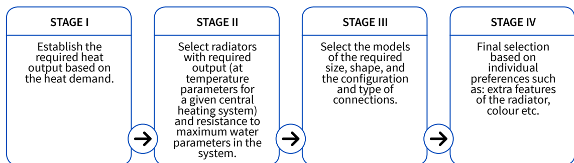
EXAMPLE RADIATOR SELECTION DIAGRAM
